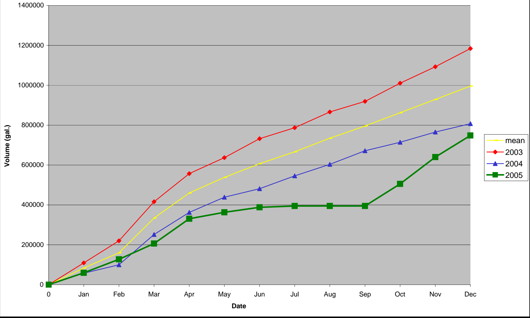
Figure 3: Historical leachate quantities at Caswell Road Landfill.
